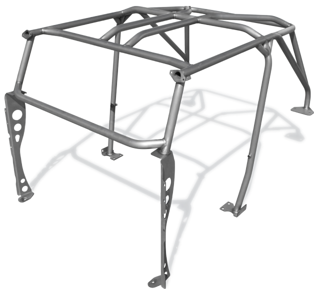
14-19-010 TJ Lazer-Fit Full Cage Kit (shown assembled)
